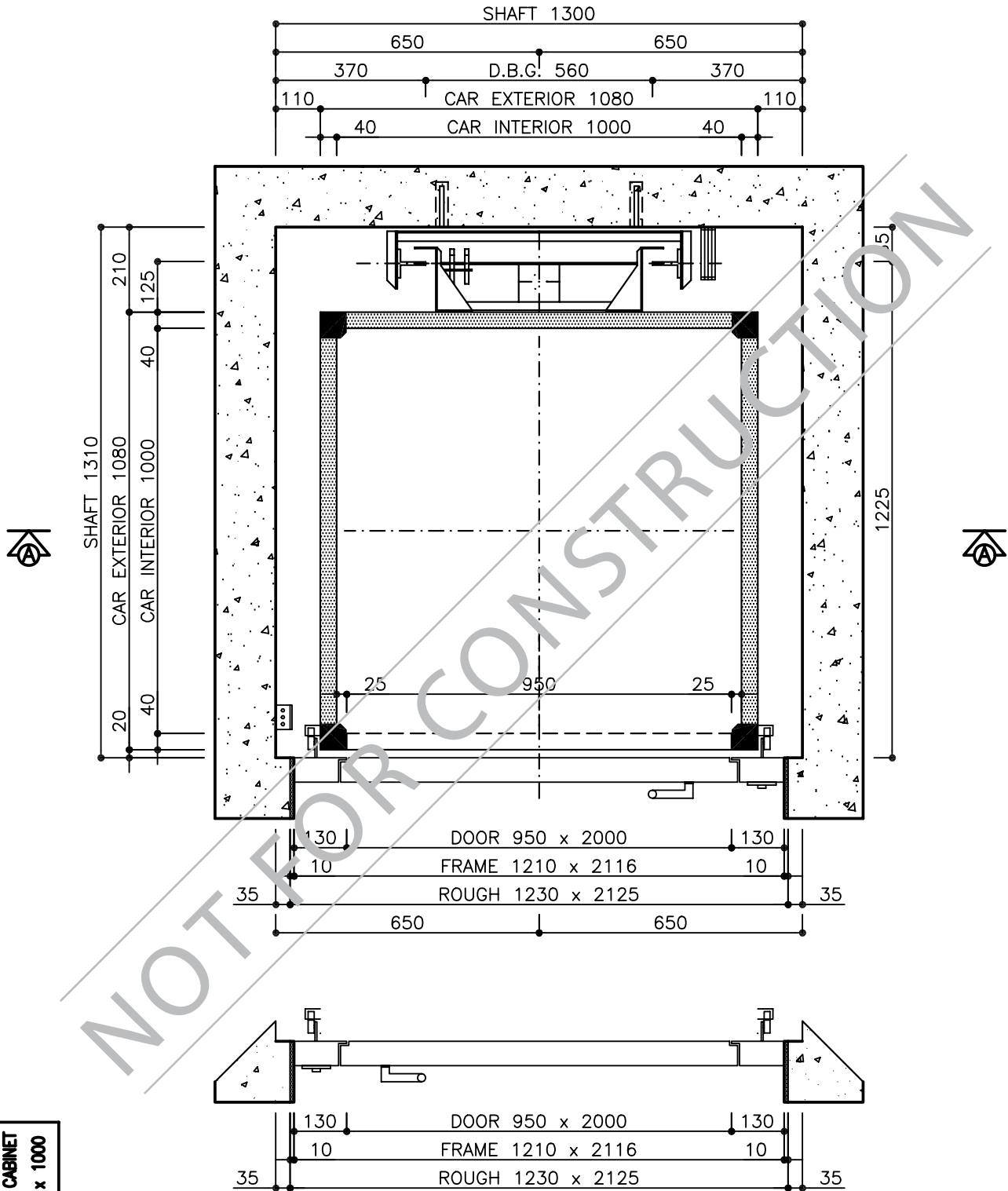
SHAFT AND CAR PLAN
